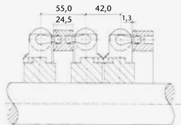
Mounting diagram
