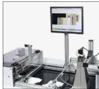
The integrated inspection camera checks every code for quality and readability and ensures, if necessary the ejection by the waste gate. All events are reported to the database of Unique Code Software.
