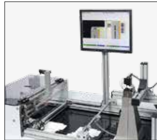
The integrated inspection camera checks every code for quality and readability and ensures, if necessary the ejection by the waste gate.
